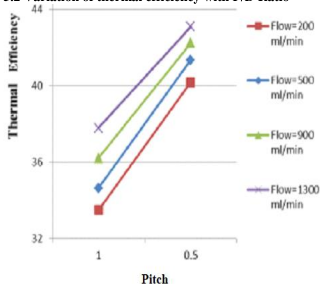
Fig.1: Variation of Thermal efficiency with pitch
