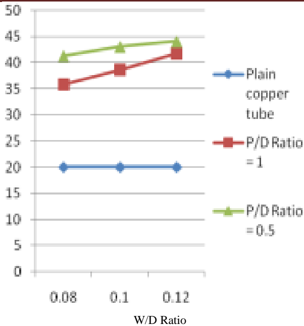
Fig. 2: Thermal Efficiency with Flow rate @ 500ml/min
