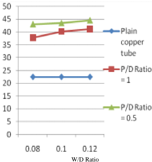
Fig. 3: Thermal Efficiency with Flow rate @ 1300ml/min
